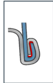
Double Seam
